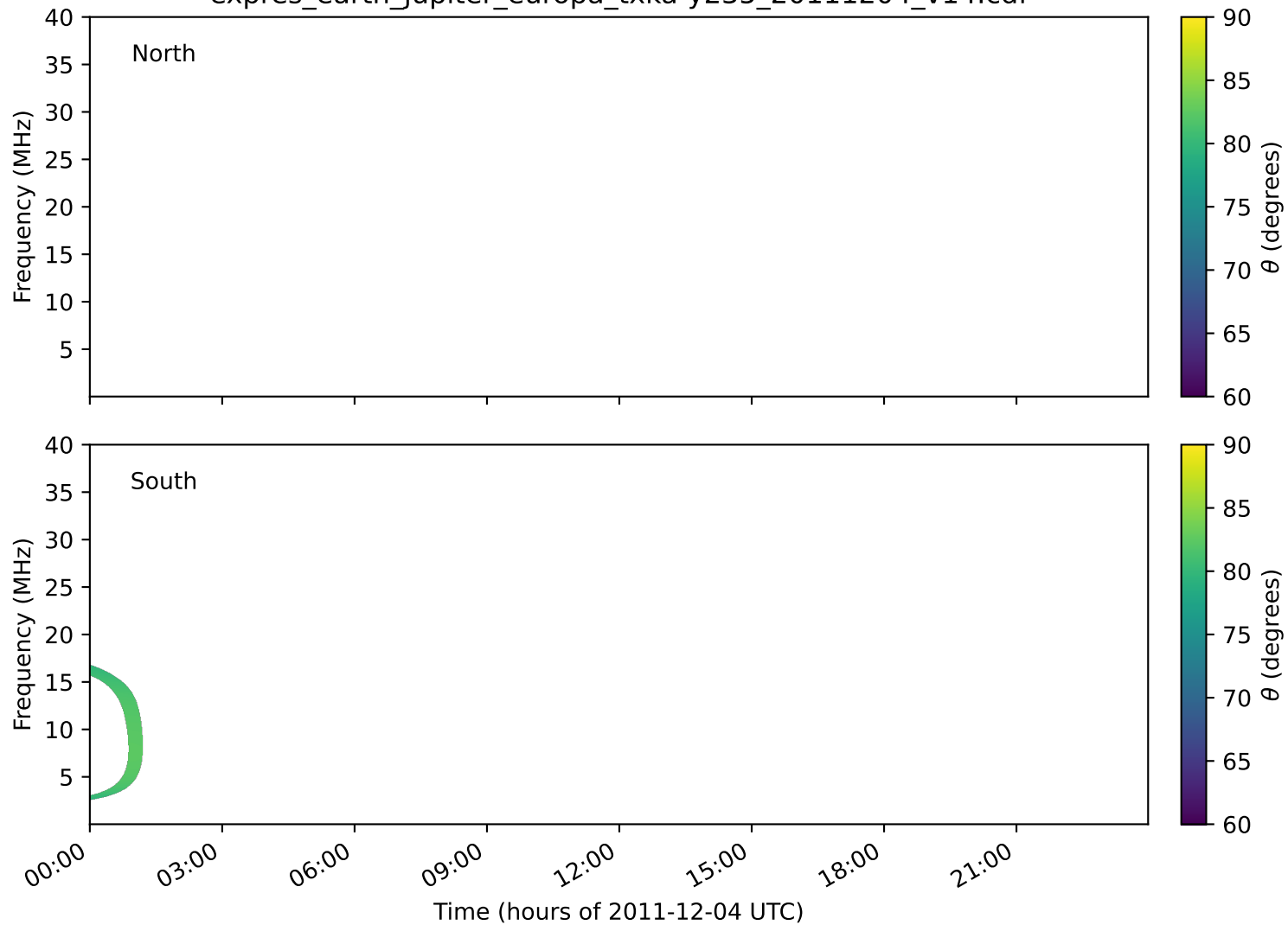
expres_earth_jupiter_europa_txka-y235_20111204_v14.cdf
