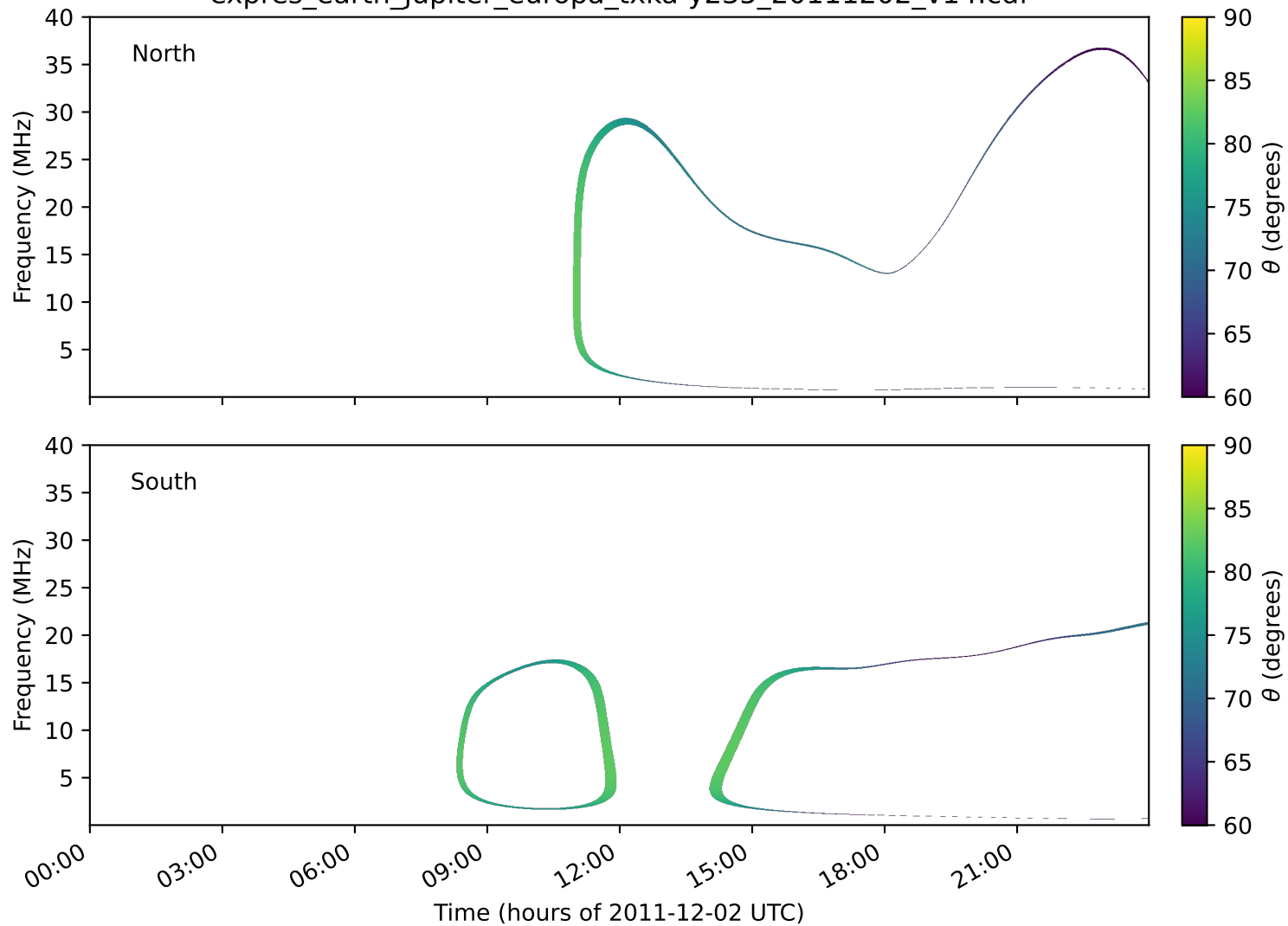
expres_earth_jupiter_europa_txka-y235_20111202_v14.cdf
