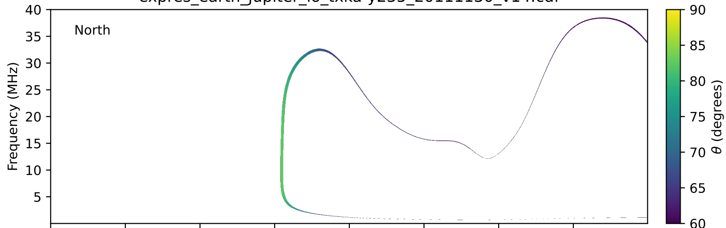
expres_earth_jupiter_io_txka-y235_20111130_v14.cdf
