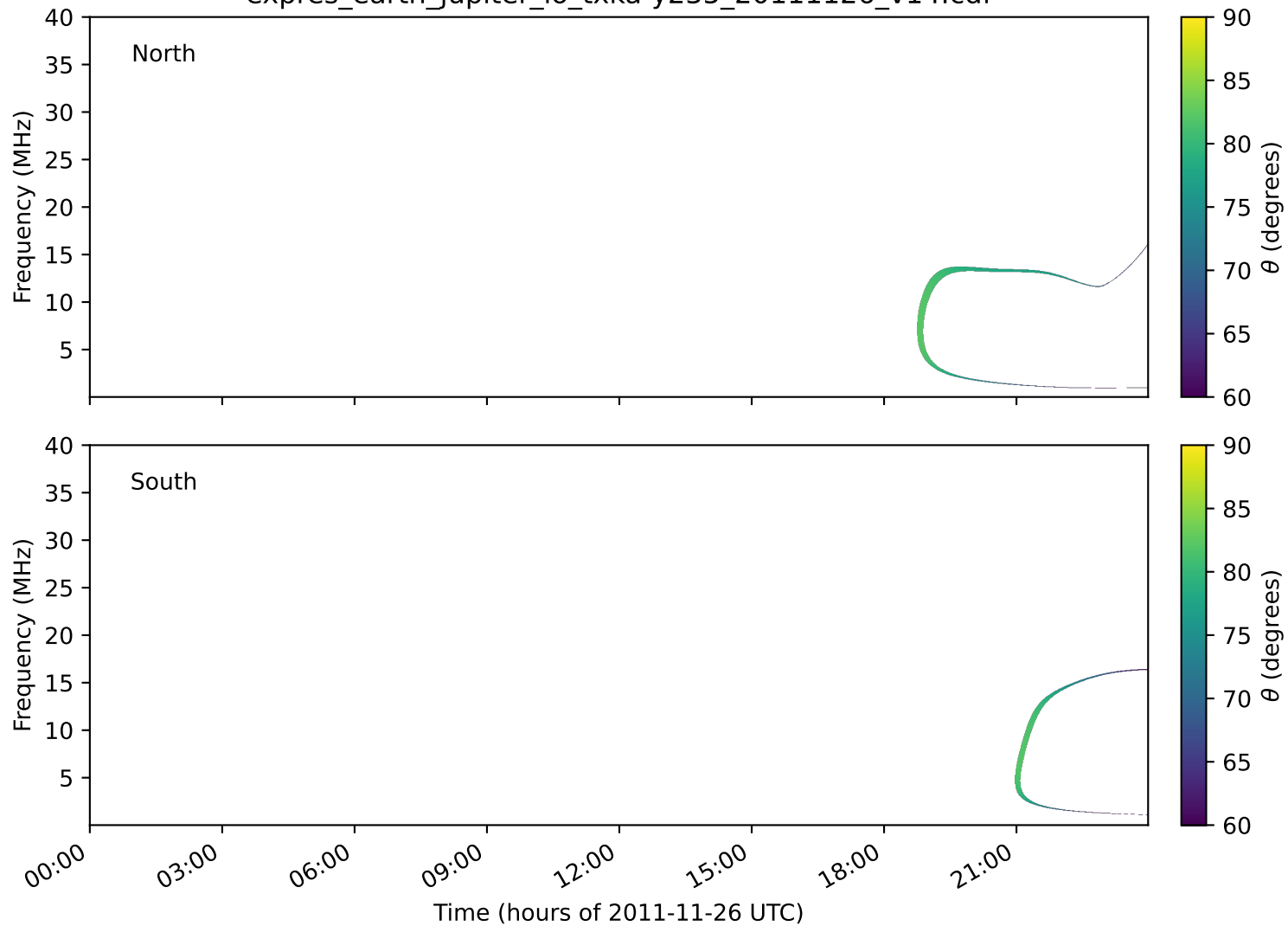
expres_earth_jupiter_io_txka-y235_20111126_v14.cdf
