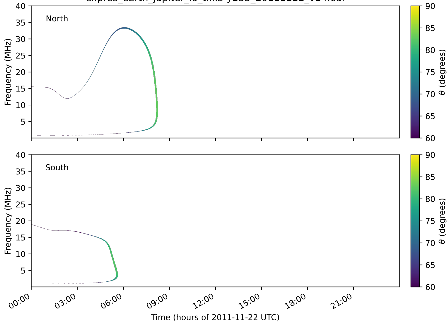
expres_earth_jupiter_io_txka-y235_20111122_v14.cdf
