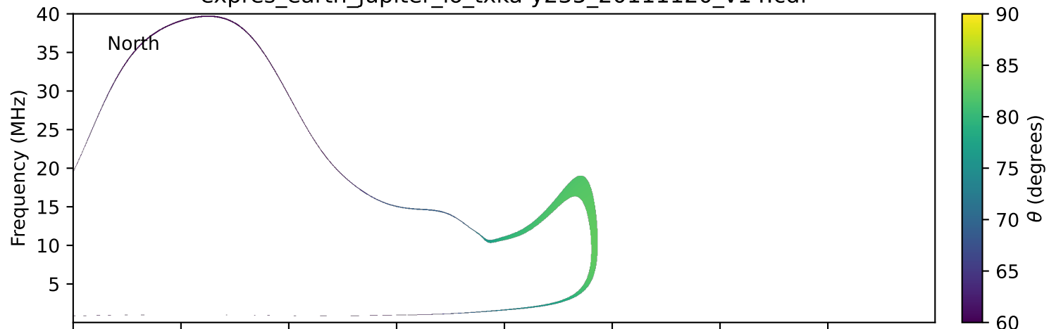
expres_earth_jupiter_io_txka-y235_20111120_v14.cdf
