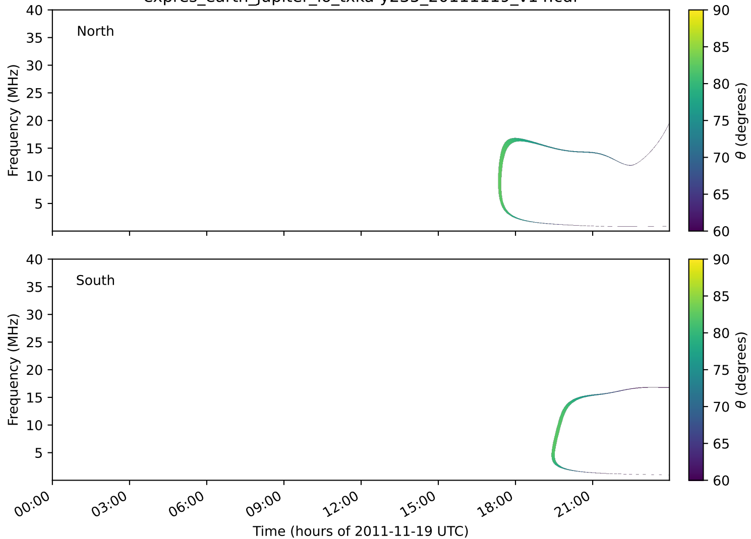
expres_earth_jupiter_io_txka-y235_20111119_v14.cdf
