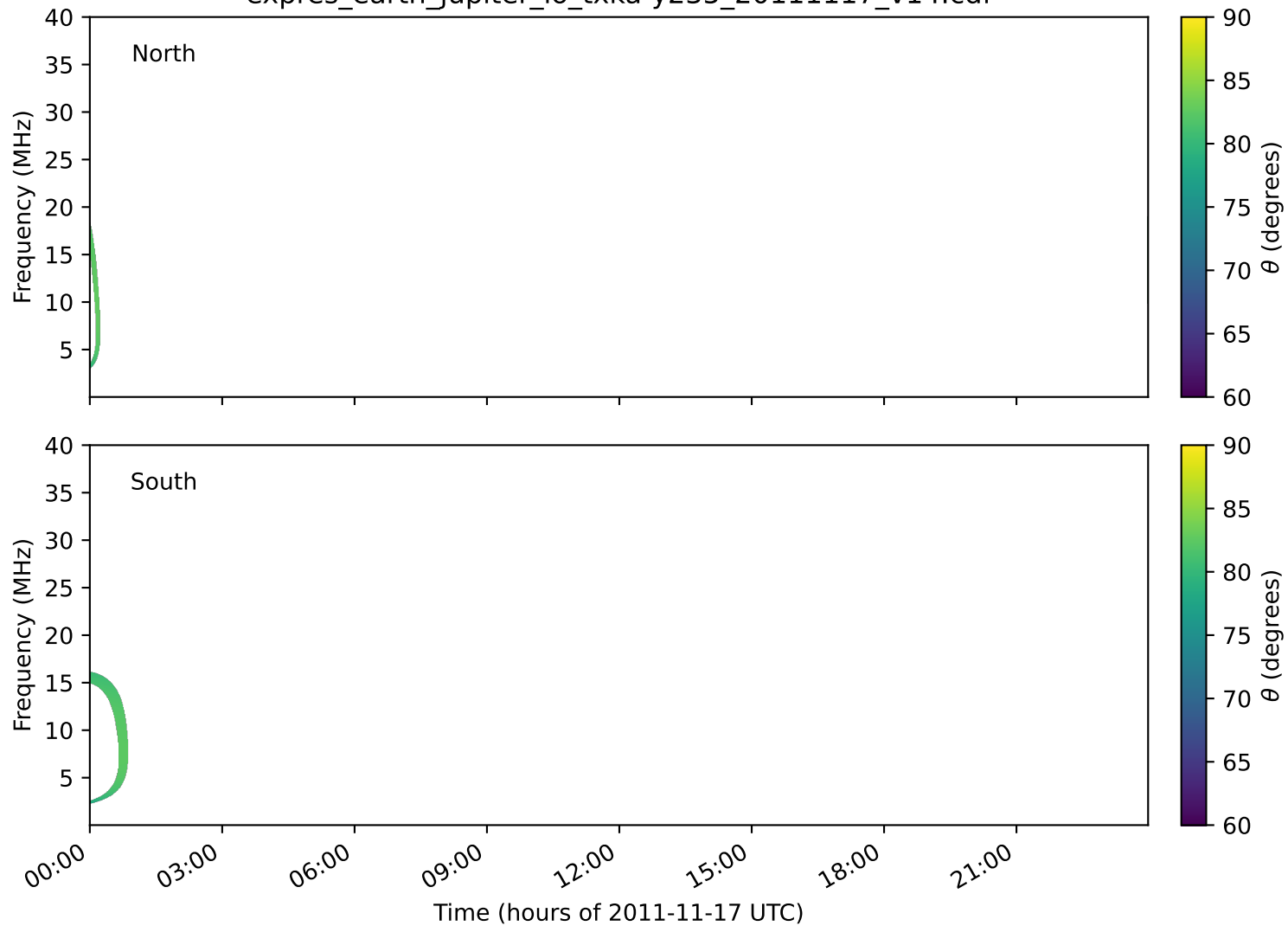
expres_earth_jupiter_io_txka-y235_20111117_v14.cdf
