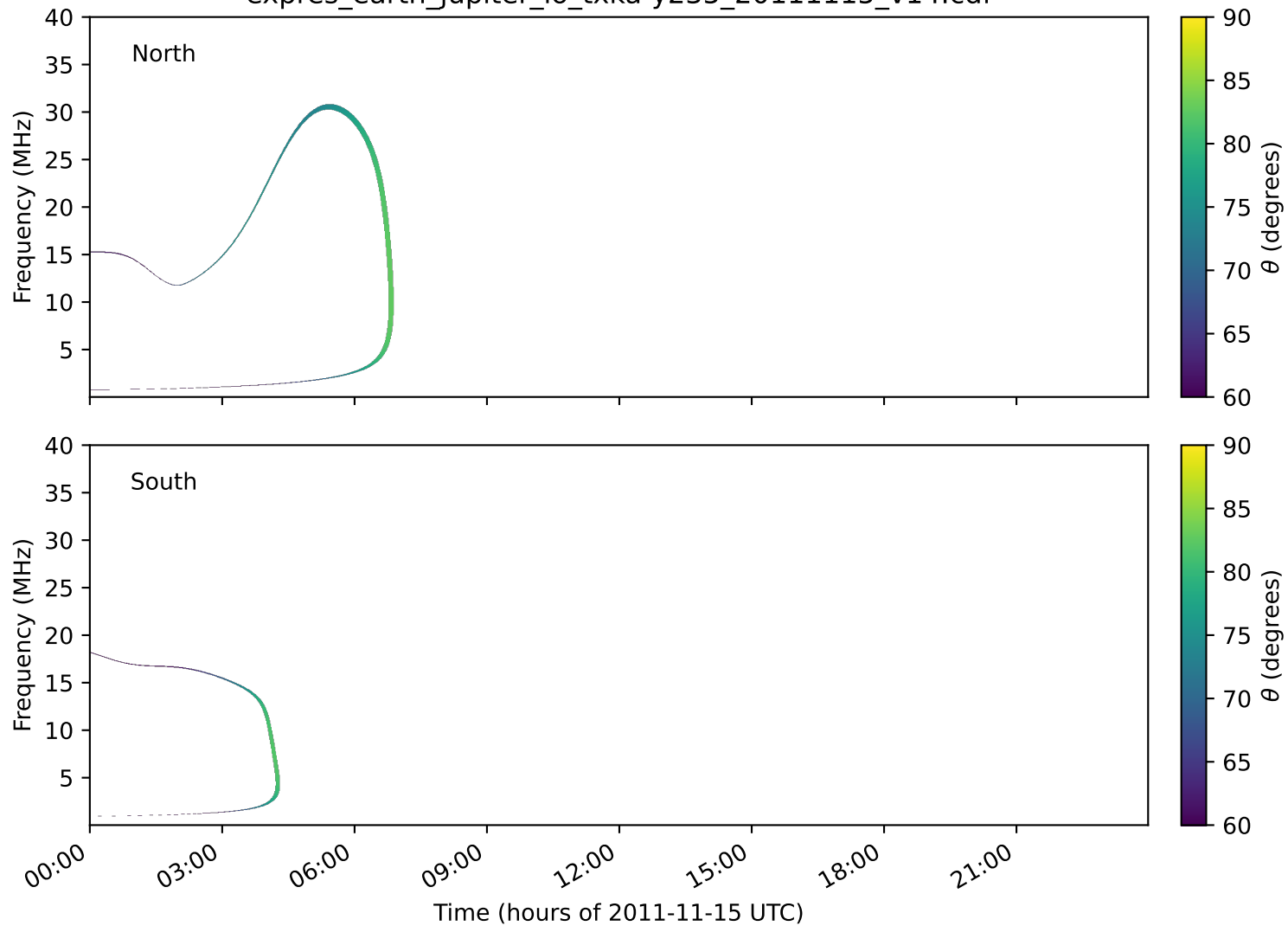
expres_earth_jupiter_io_txka-y235_20111115_v14.cdf
