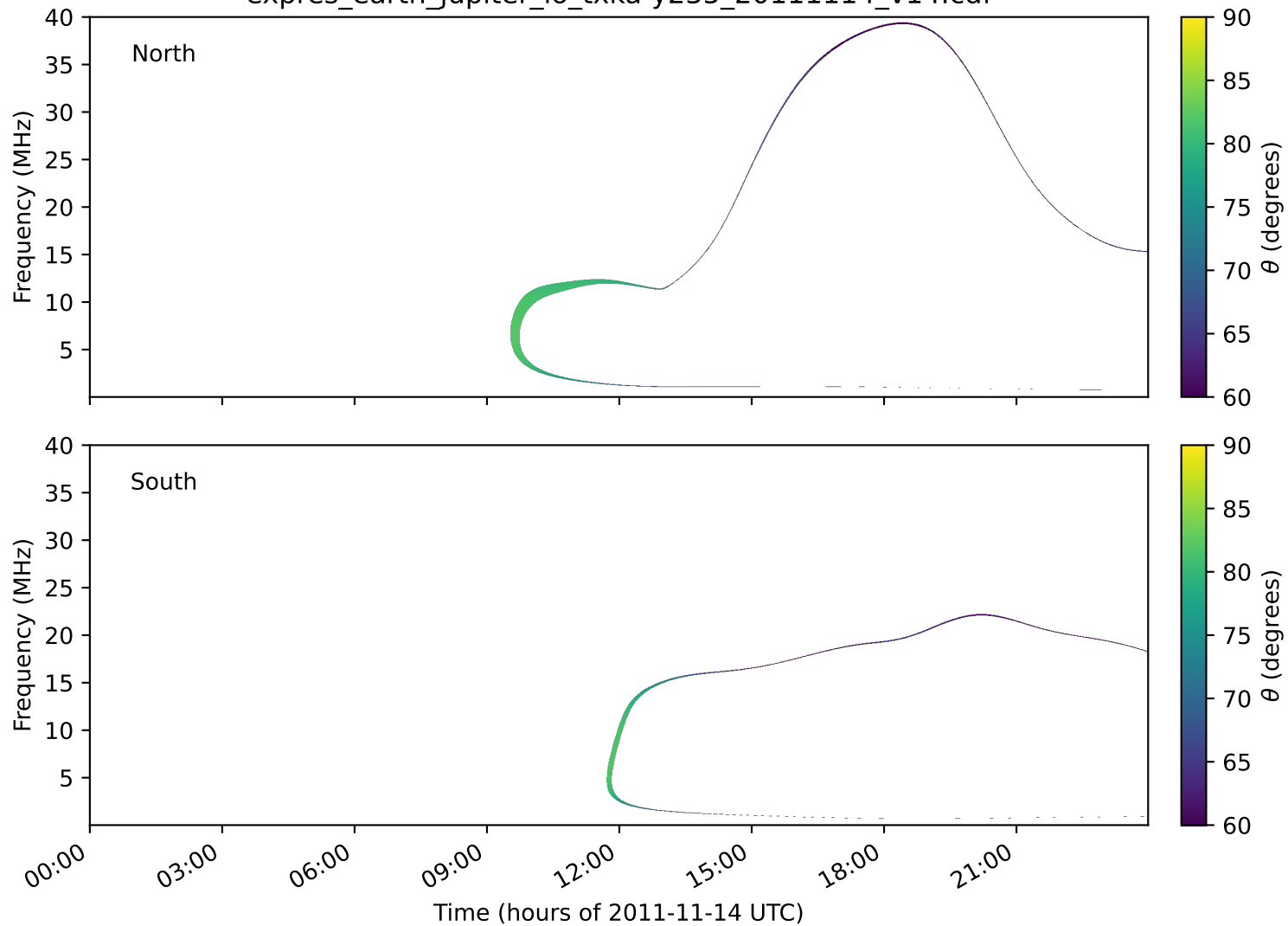
expres_earth_jupiter_io_txka-y235_20111114_v14.cdf
