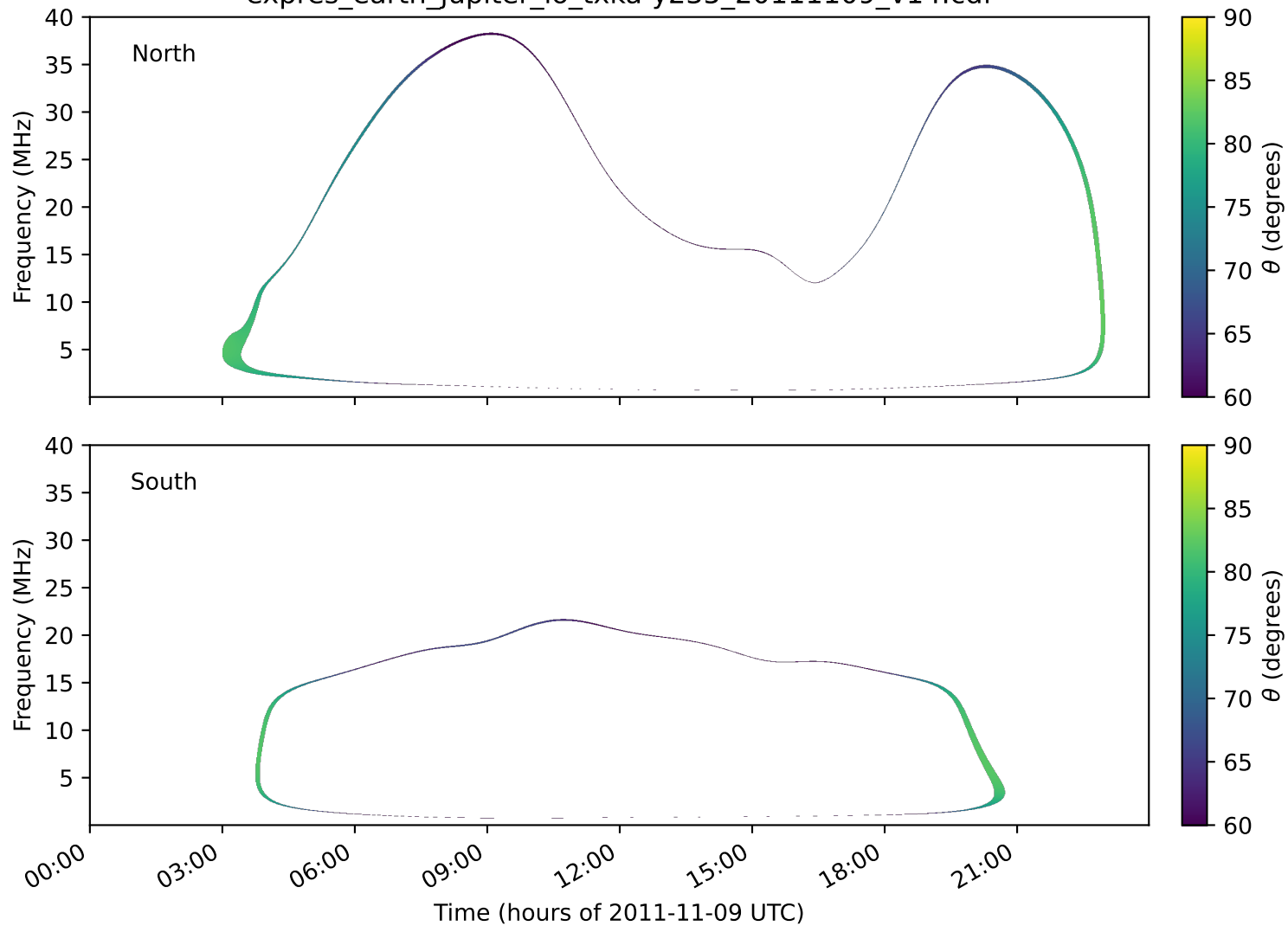
expres_earth_jupiter_io_txka-y235_20111109_v14.cdf
