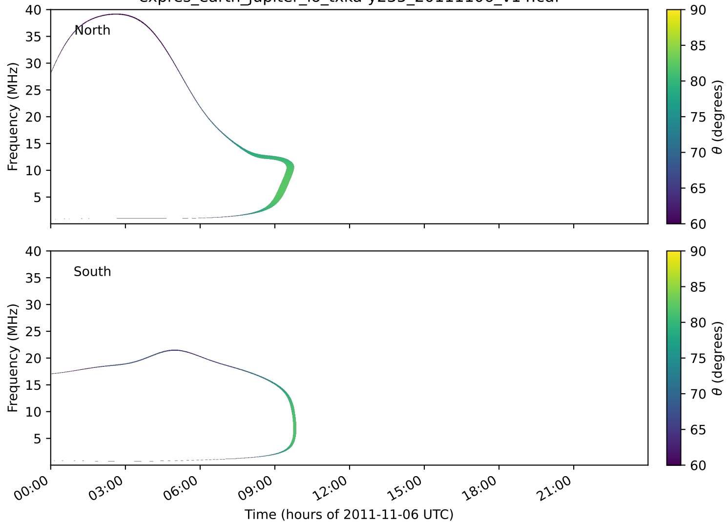
expres_earth_jupiter_io_txka-y235_20111106_v14.cdf
