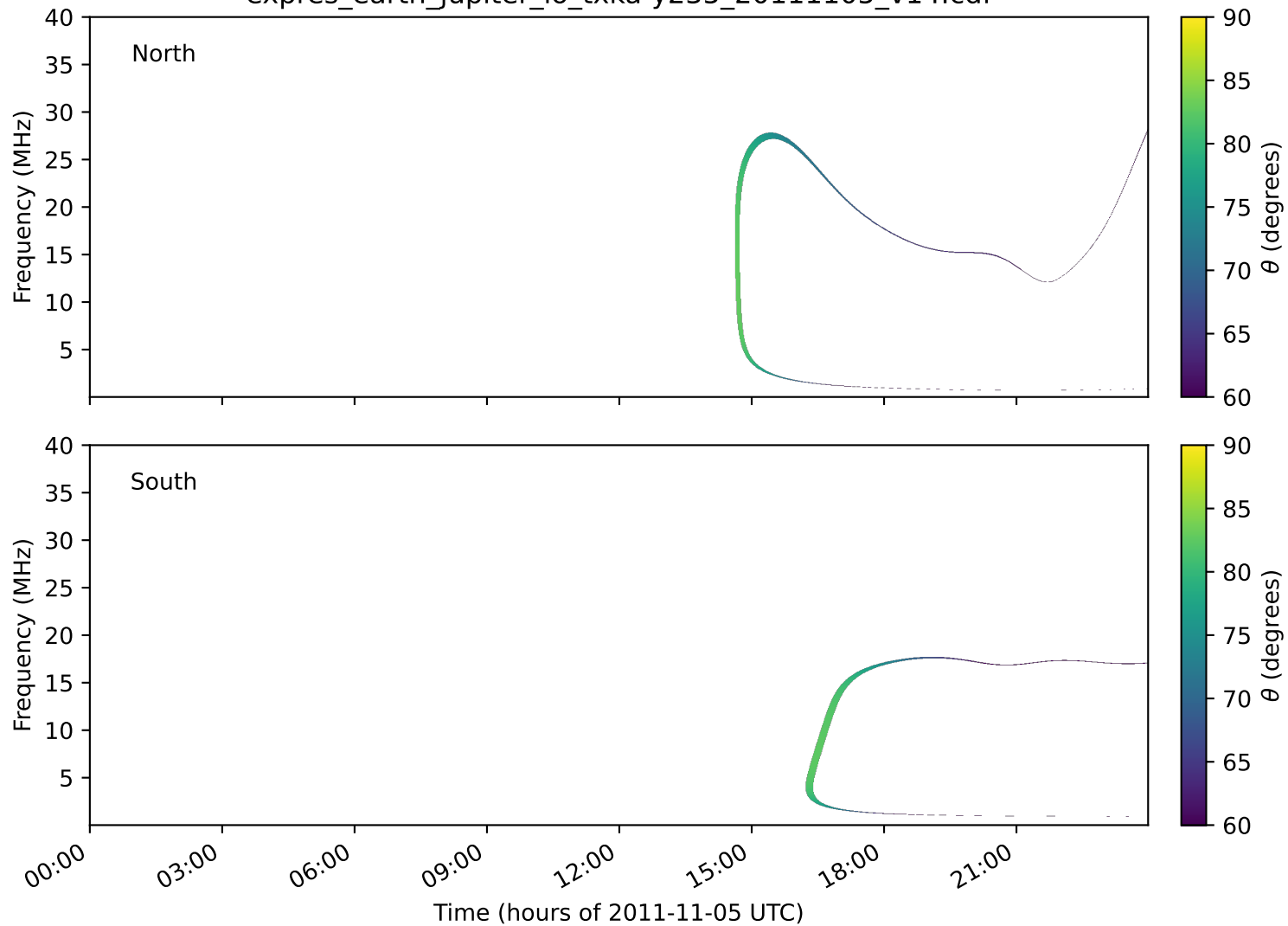
expres_earth_jupiter_io_txka-y235_20111105_v14.cdf
