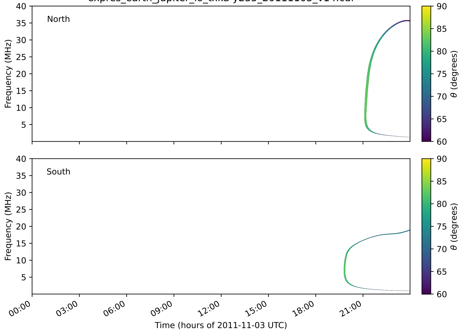
expres_earth_jupiter_io_txka-y235_20111103_v14.cdf
