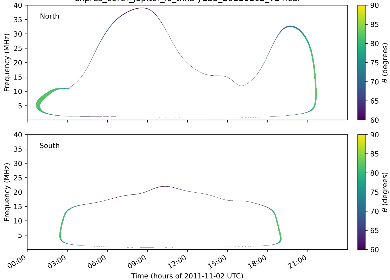
expres_earth_jupiter_io_txka-y235_20111102_v14.cdf
