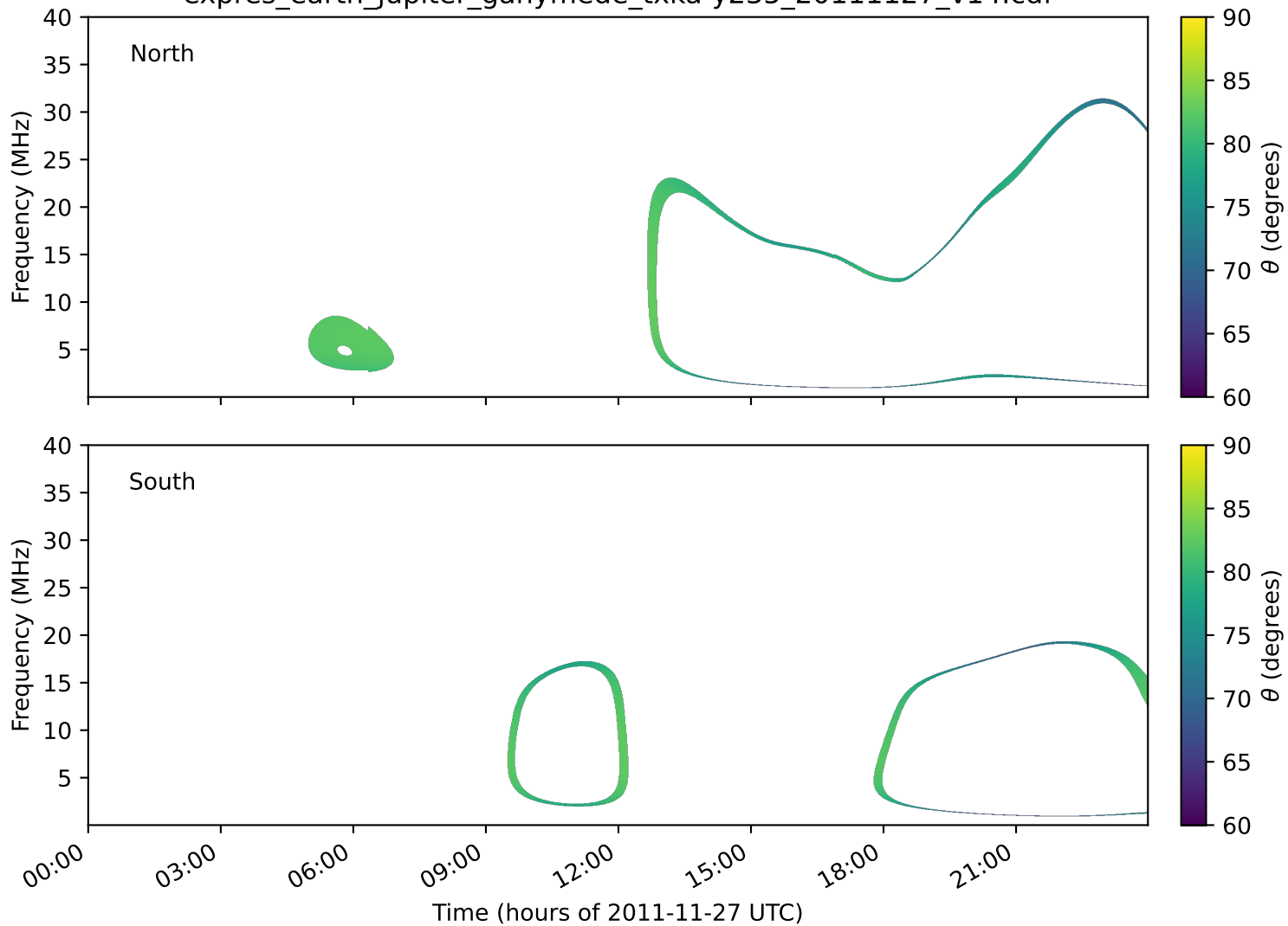
expres_earth_jupiter_ganymede_txka-y235_20111127_v14.cdf
