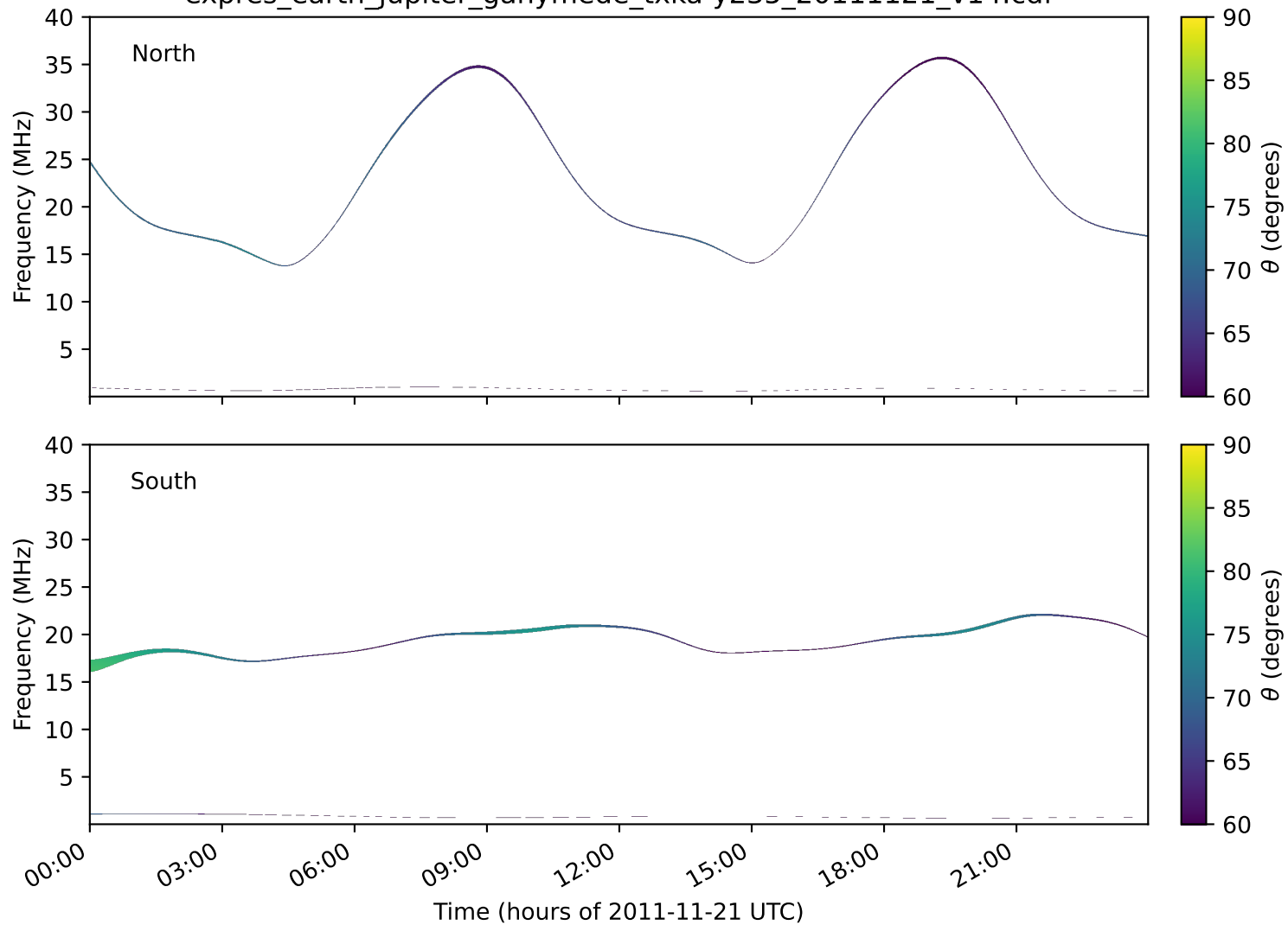
expres_earth_jupiter_ganymede_txka-y235_20111121_v14.cdf
