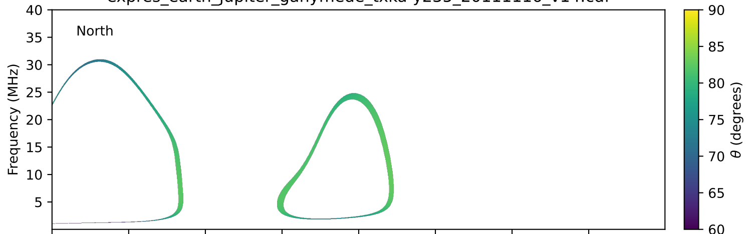
expres_earth_jupiter_ganymede_txka-y235_20111116_v14.cdf
