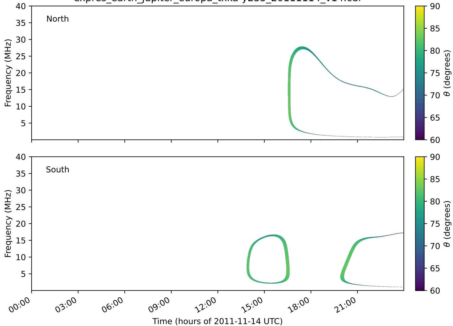
expres_earth_jupiter_europa_txka-y235_20111114_v14.cdf
