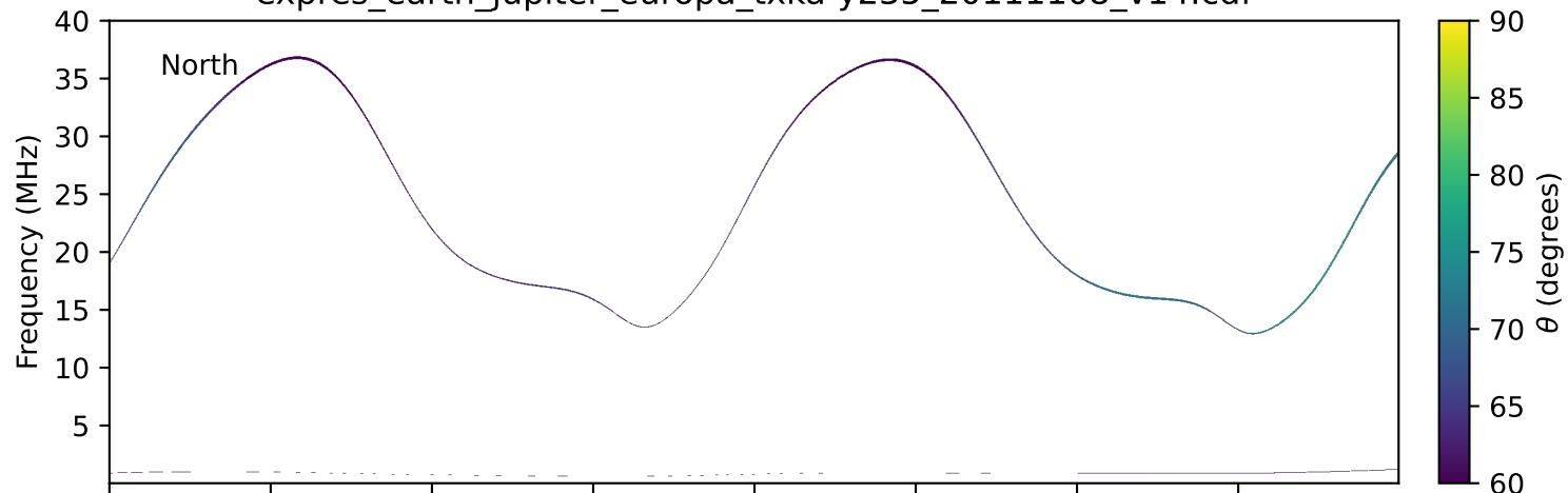
expres_earth_jupiter_europa_txka-y235_20111108_v14.cdf
