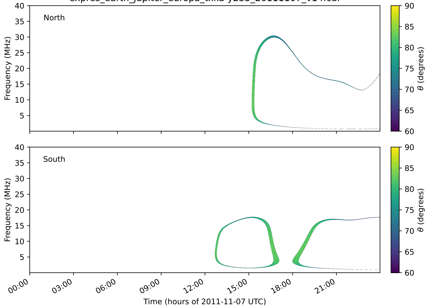
expres_earth_jupiter_europa_txka-y235_20111107_v14.cdf
