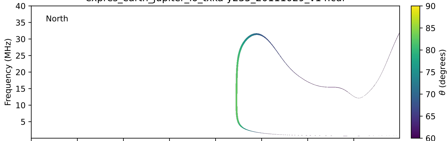
expres_earth_jupiter_io_txka-y235_20111029_v14.cdf
