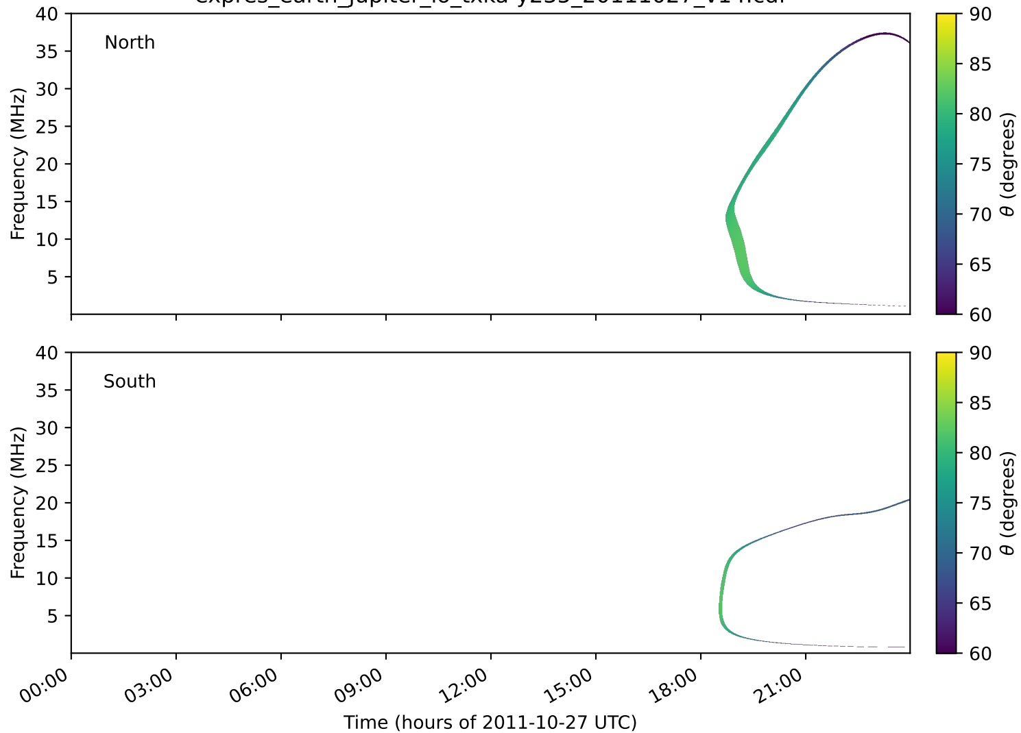
expres_earth_jupiter_io_txka-y235_20111027_v14.cdf
