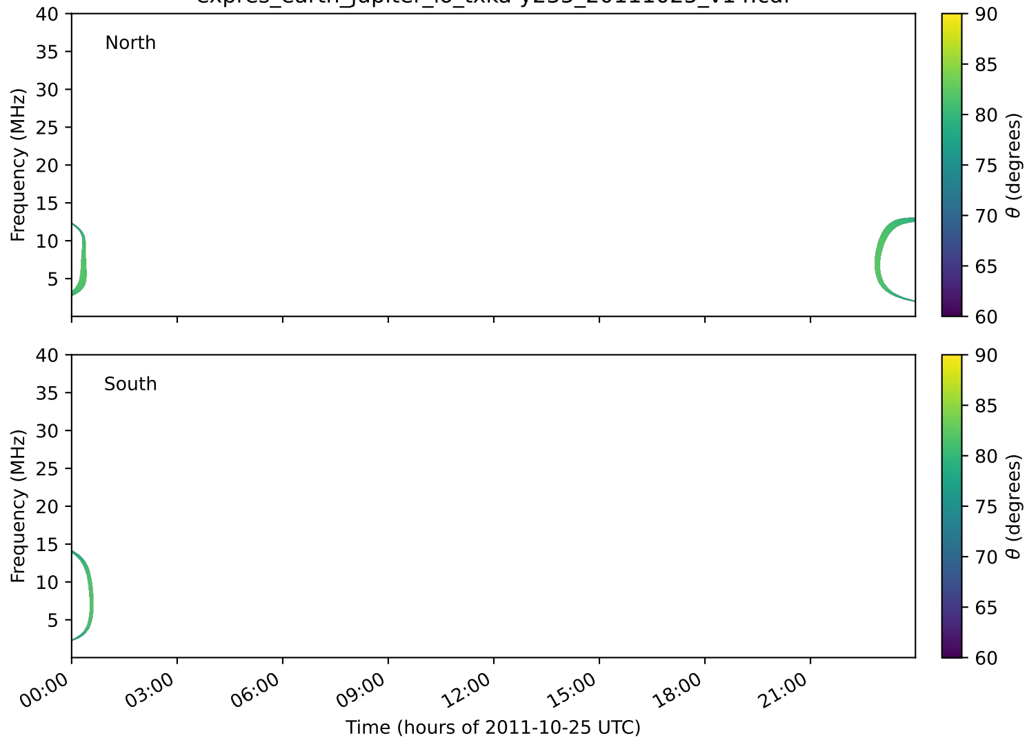
expres_earth_jupiter_io_txka-y235_20111025_v14.cdf
