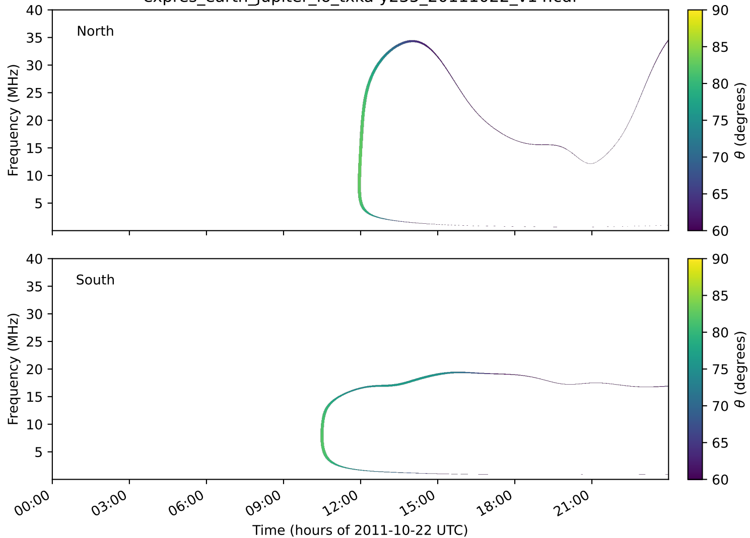
expres_earth_jupiter_io_txka-y235_20111022_v14.cdf
