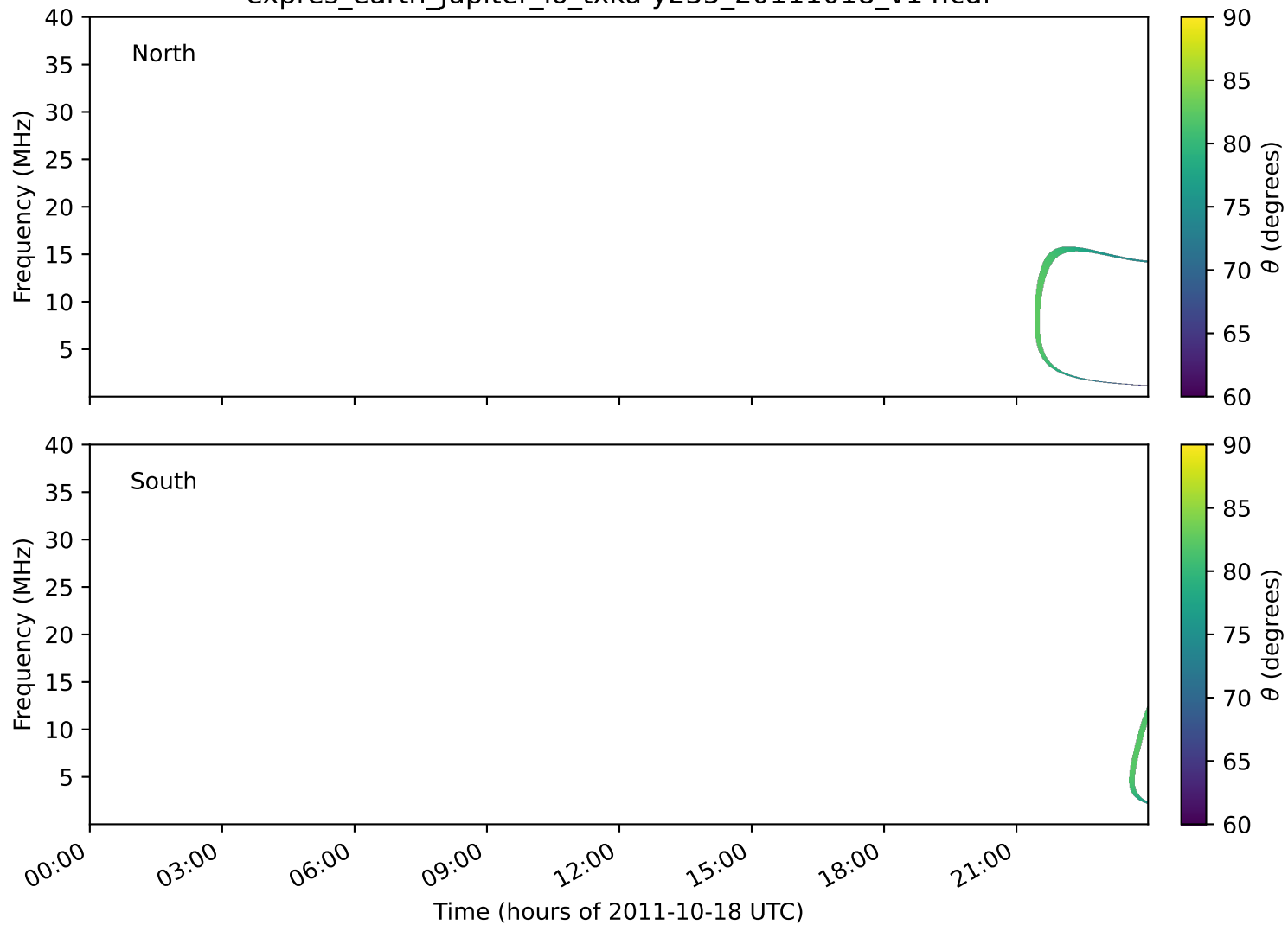
expres_earth_jupiter_io_txka-y235_20111018_v14.cdf
