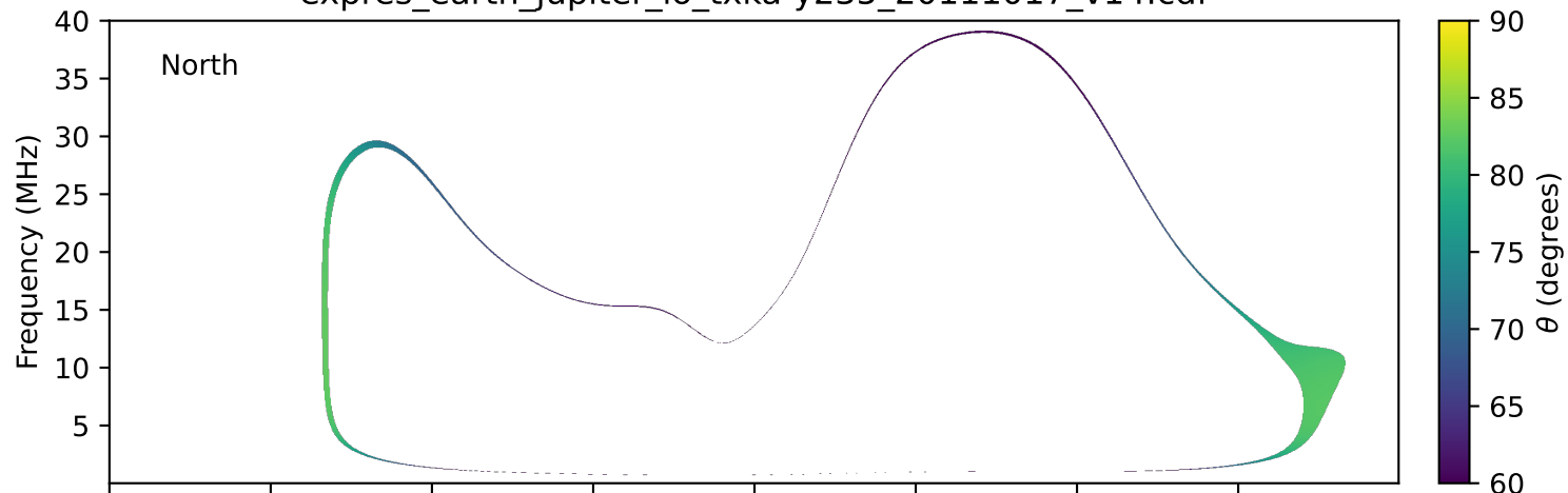
expres_earth_jupiter_io_txka-y235_20111017_v14.cdf
