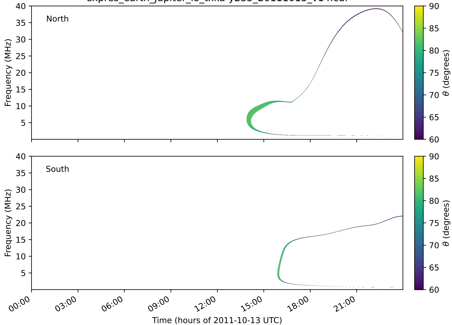
expres_earth_jupiter_io_txka-y235_20111013_v14.cdf
