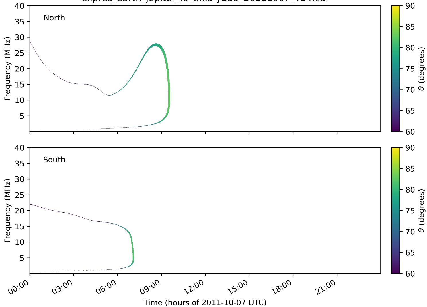
expres_earth_jupiter_io_txka-y235_20111007_v14.cdf
