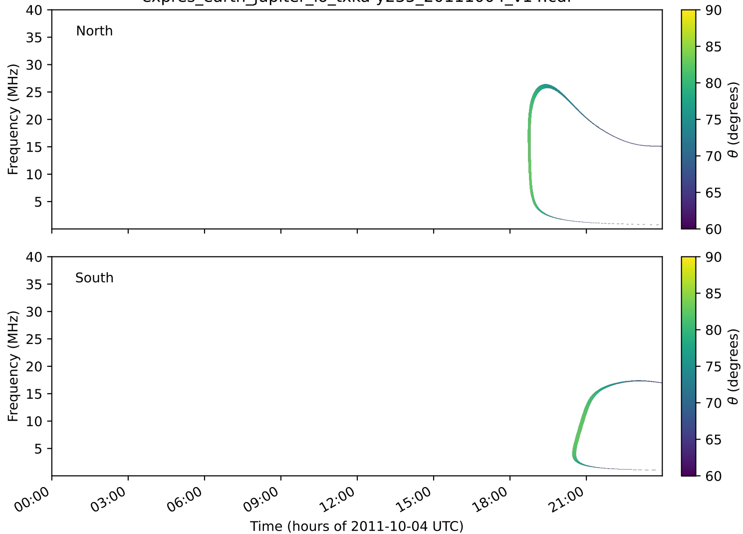
expres_earth_jupiter_io_txka-y235_20111004_v14.cdf
