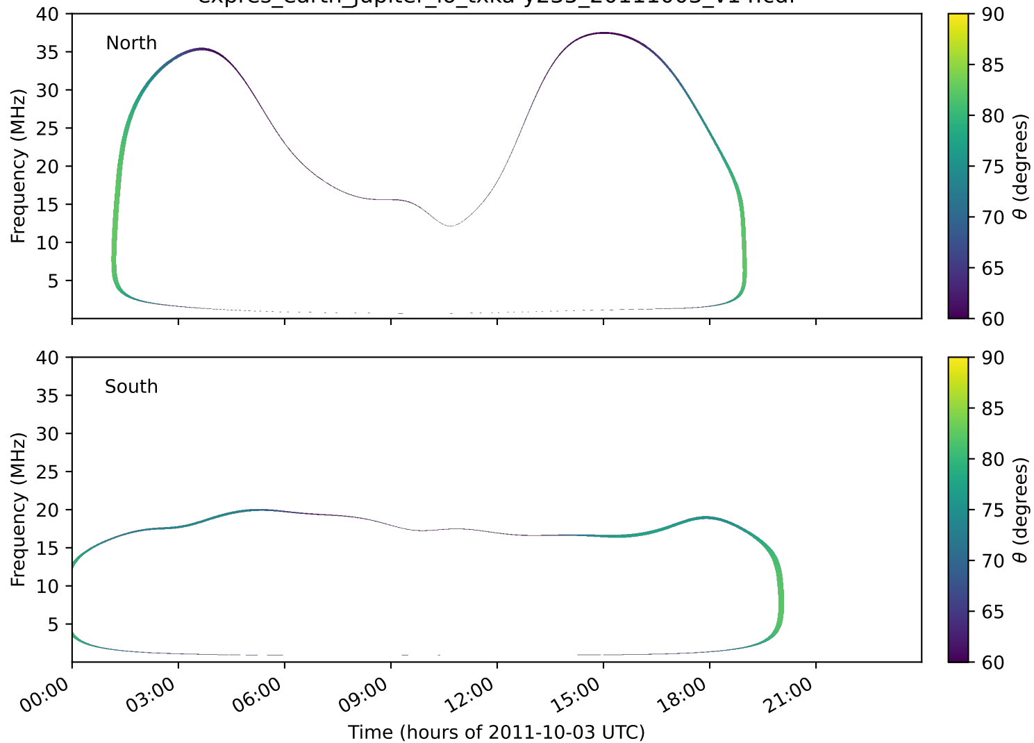
expres_earth_jupiter_io_txka-y235_20111003_v14.cdf
