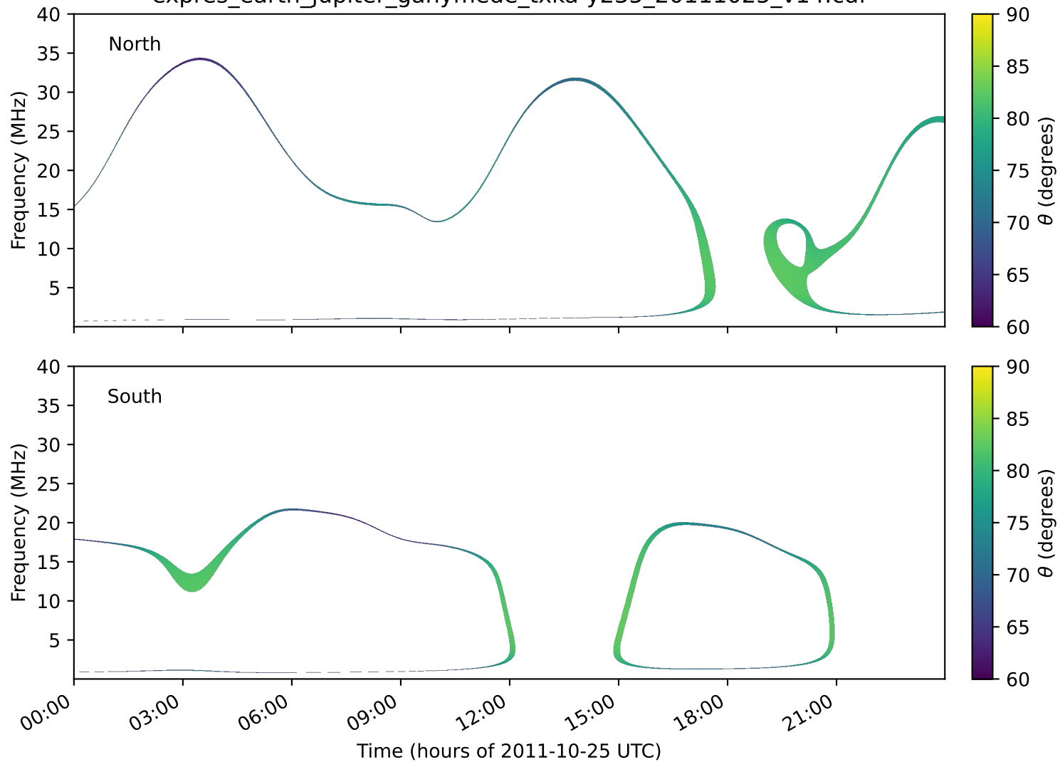
expres_earth_jupiter_ganymede_txka-y235_20111025_v14.cdf
