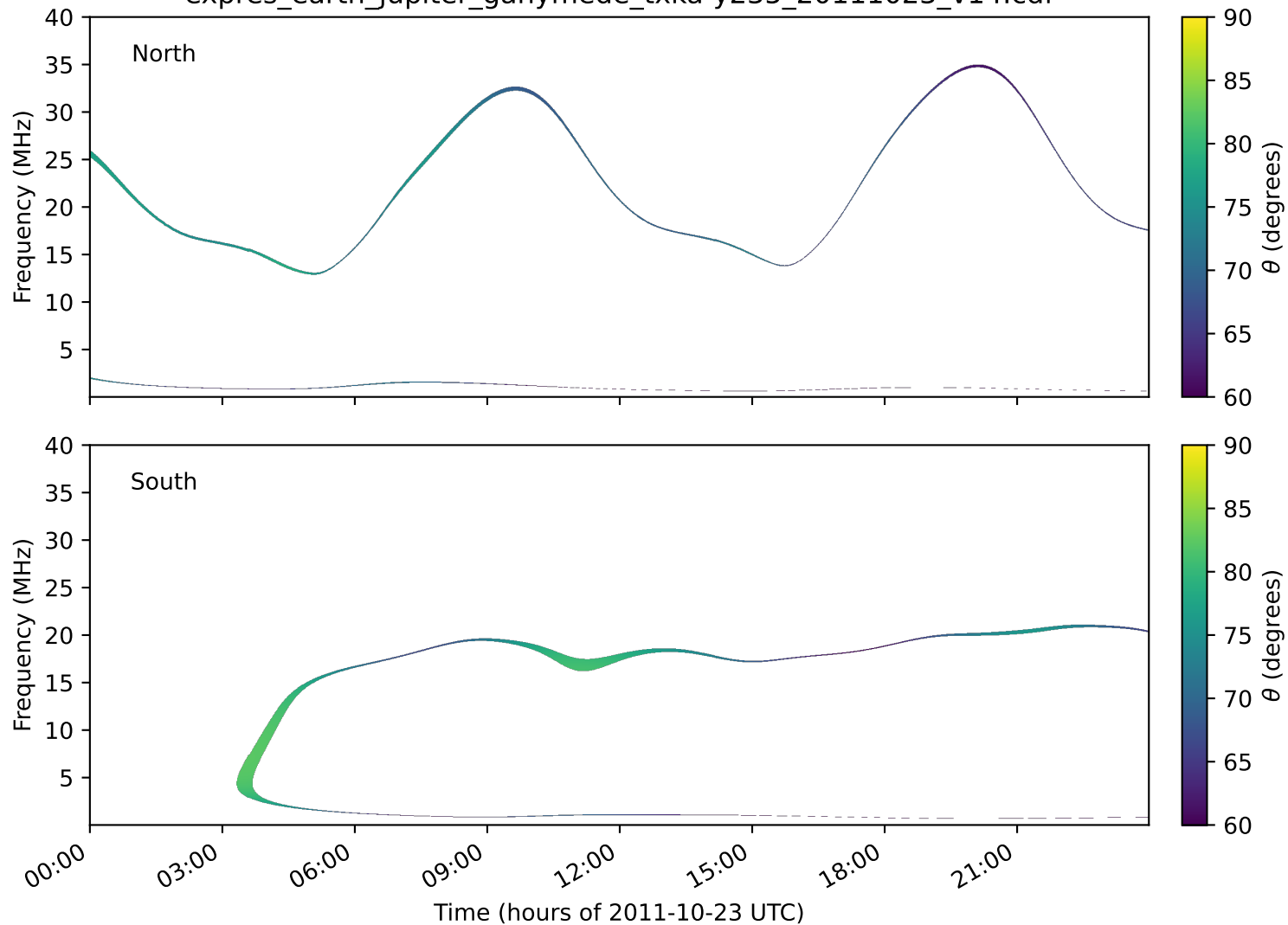
expres_earth_jupiter_ganymede_txka-y235_20111023_v14.cdf
