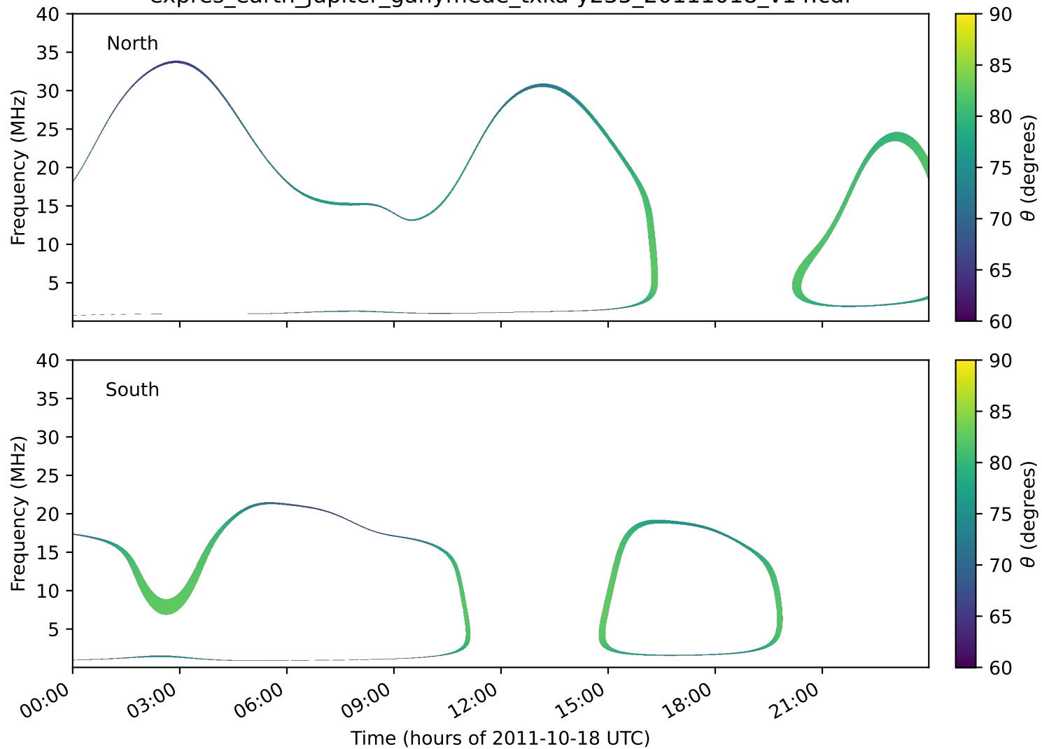
expres_earth_jupiter_ganymede_txka-y235_20111018_v14.cdf
