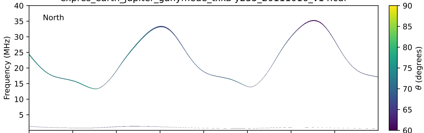
expres_earth_jupiter_ganymede_txka-y235_20111016_v14.cdf
