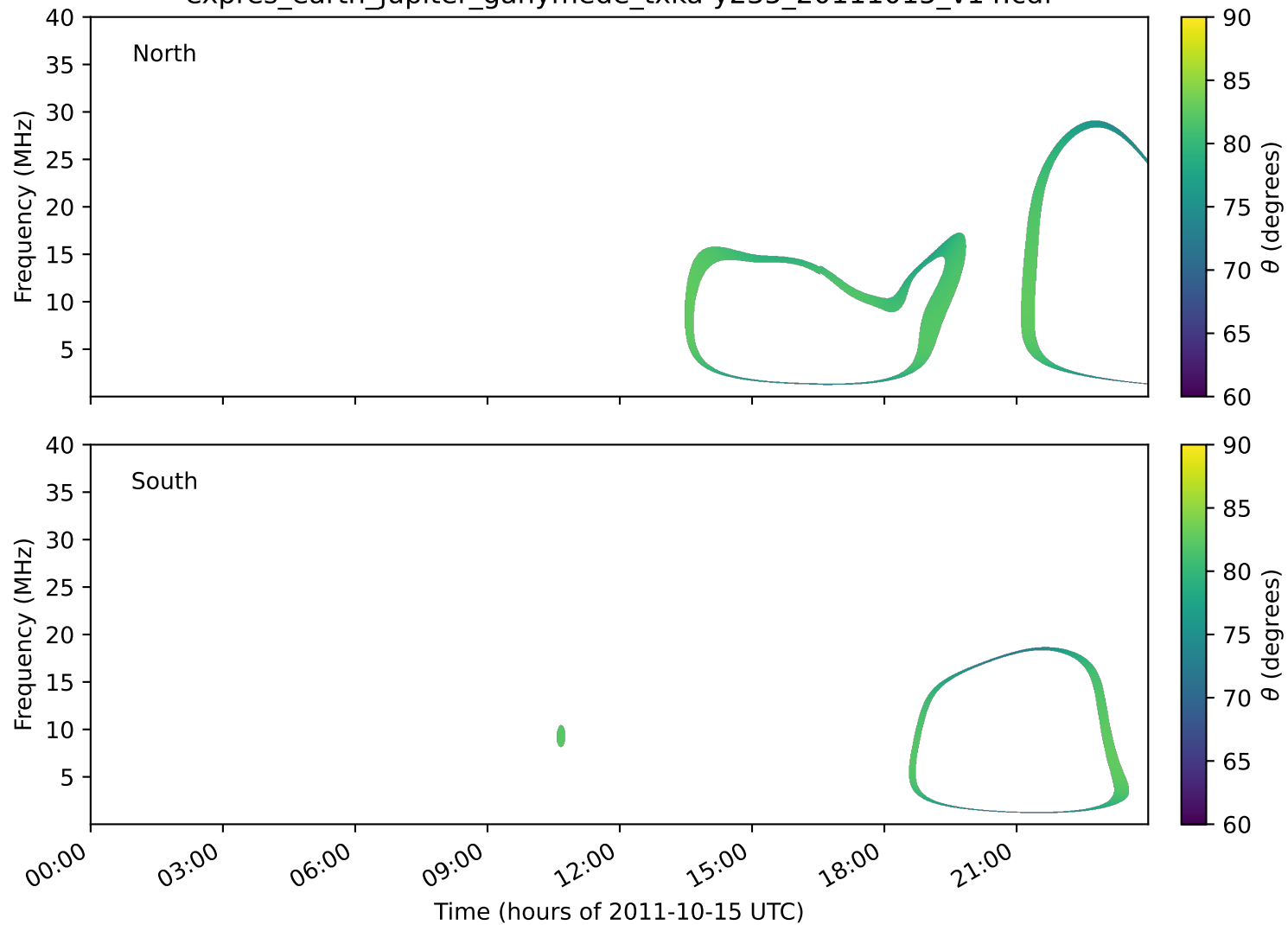
expres_earth_jupiter_ganymede_txka-y235_20111015_v14.cdf
