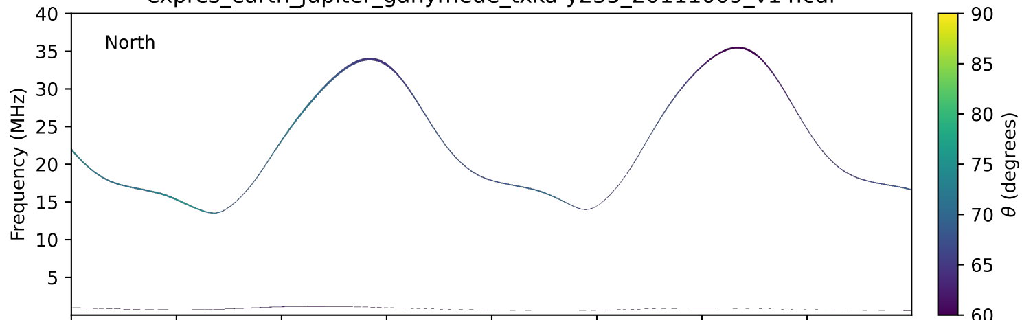
expres_earth_jupiter_ganymede_txka-y235_20111009_v14.cdf
