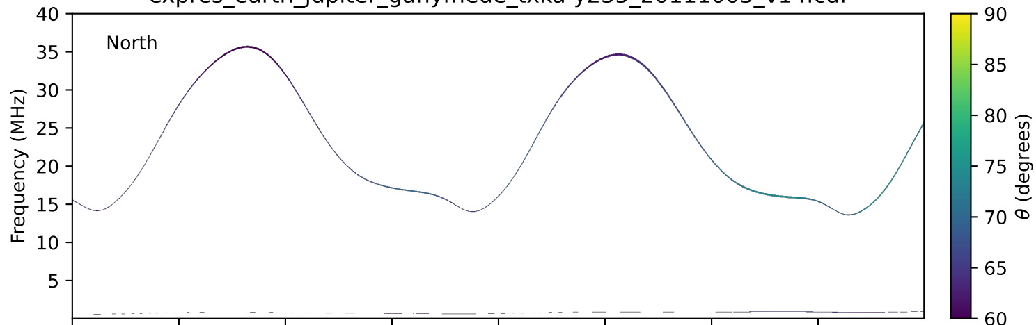
expres_earth_jupiter_ganymede_txka-y235_20111003_v14.cdf
