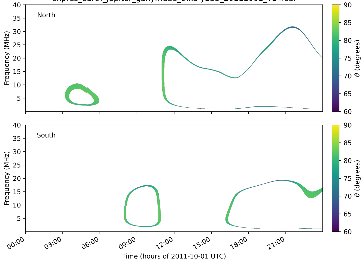
expres_earth_jupiter_ganymede_txka-y235_20111001_v14.cdf
