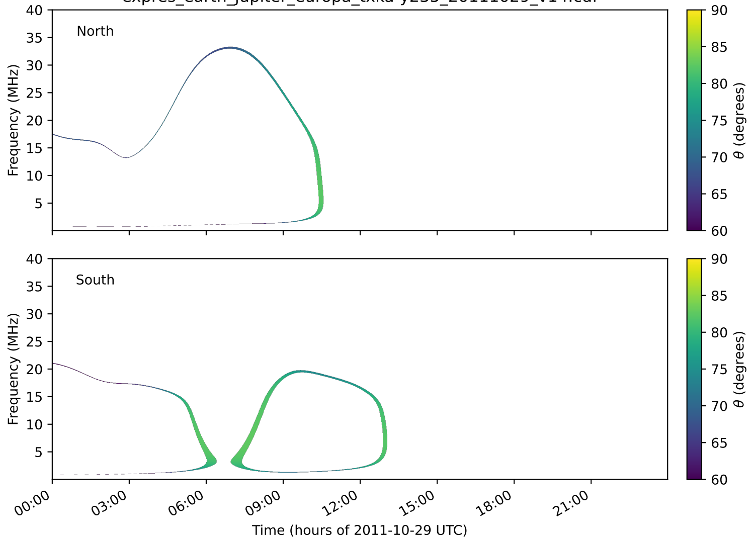
expres_earth_jupiter_europa_txka-y235_20111029_v14.cdf
