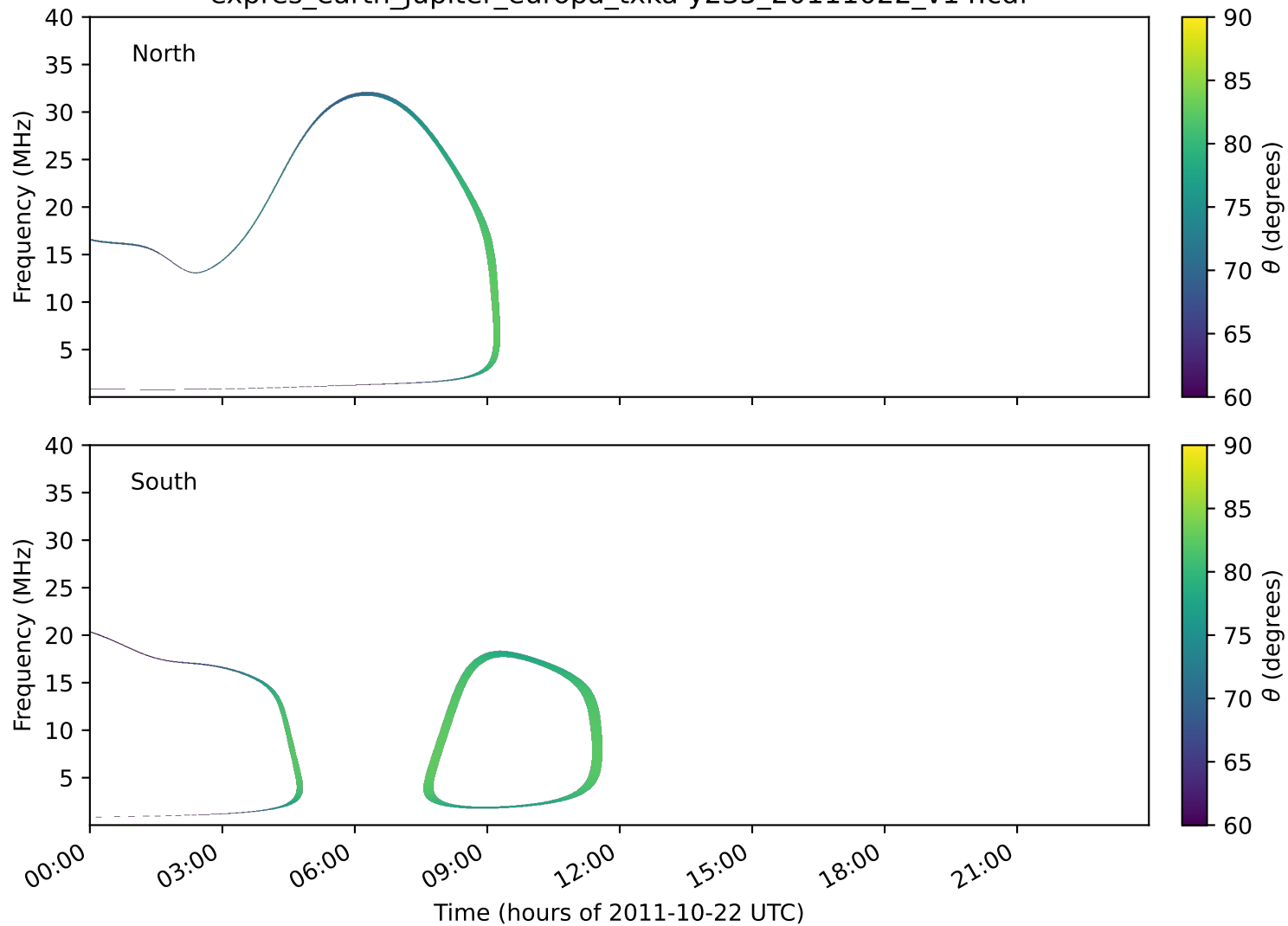
expres_earth_jupiter_europa_txka-y235_20111022_v14.cdf
