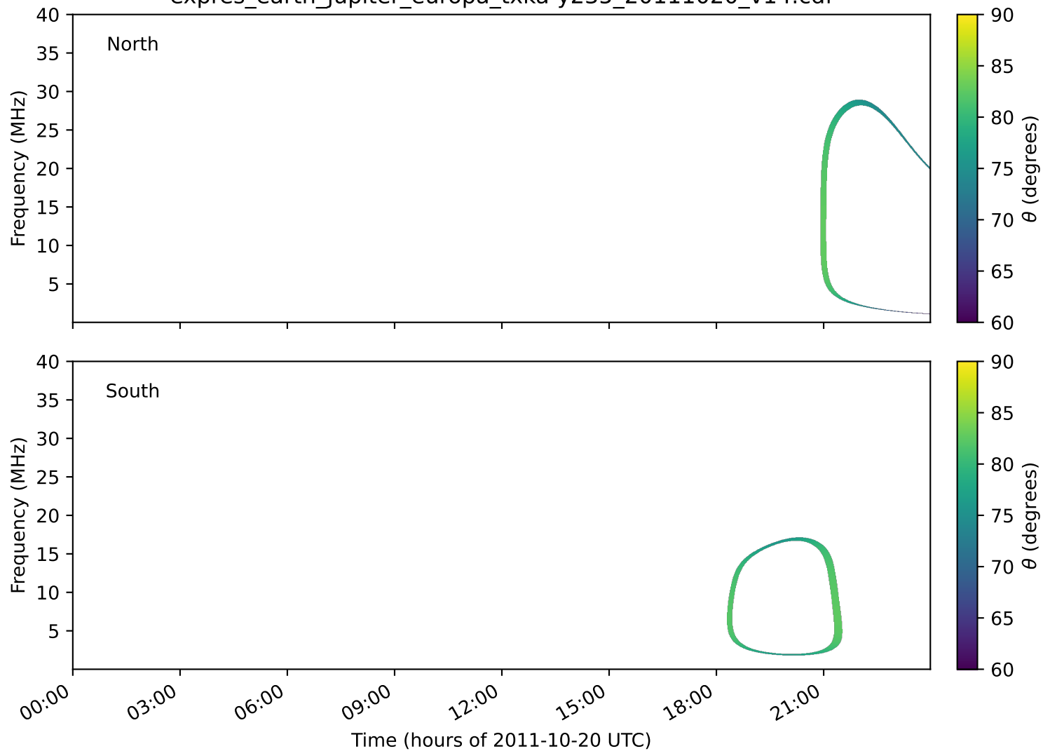
expres_earth_jupiter_europa_txka-y235_20111020_v14.cdf
