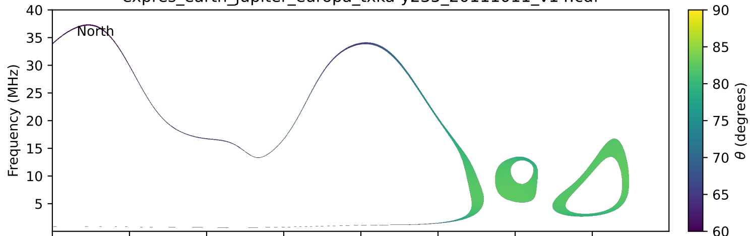
expres_earth_jupiter_europa_txka-y235_20111011_v14.cdf
