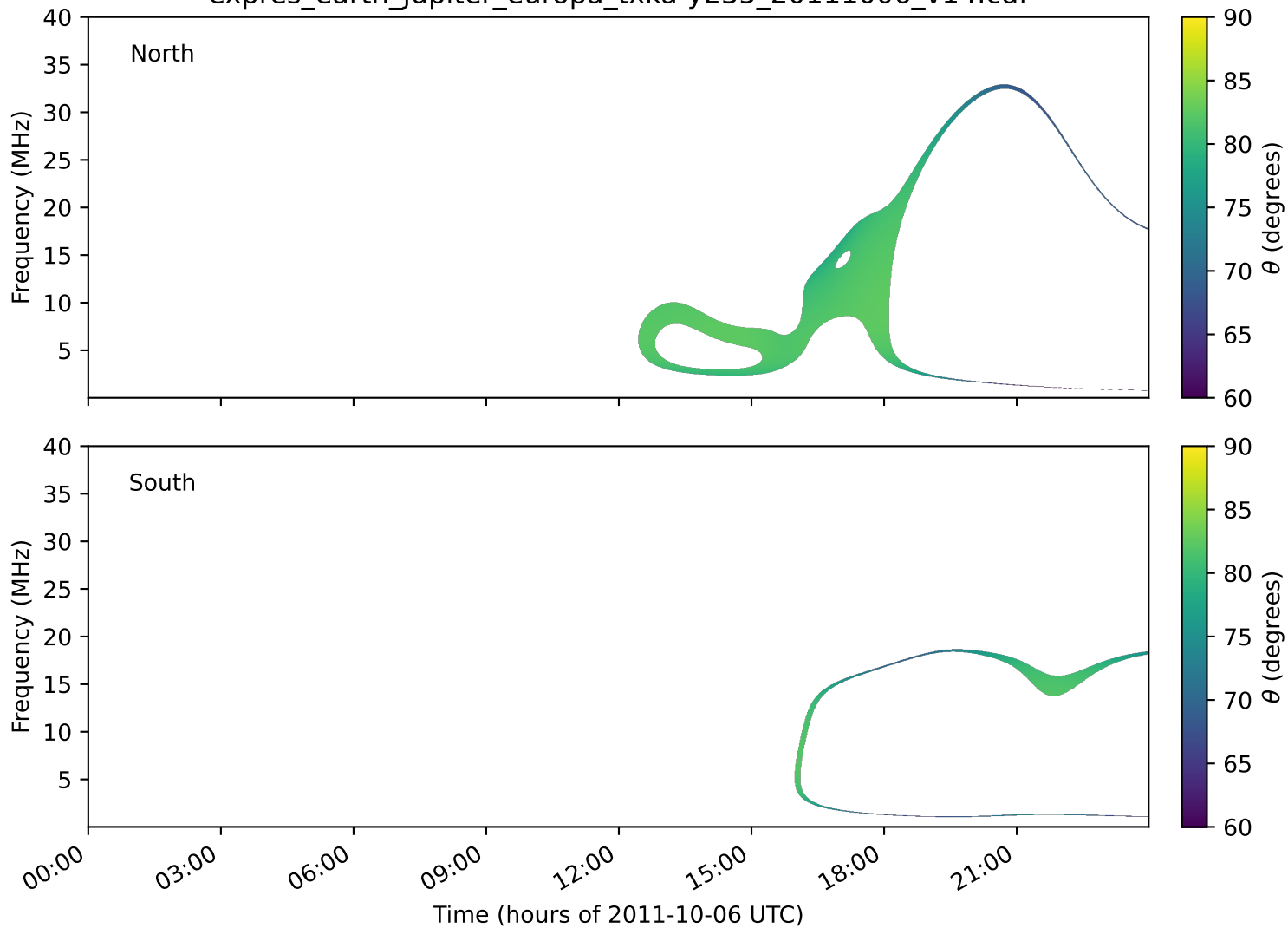
expres_earth_jupiter_europa_txka-y235_20111006_v14.cdf
