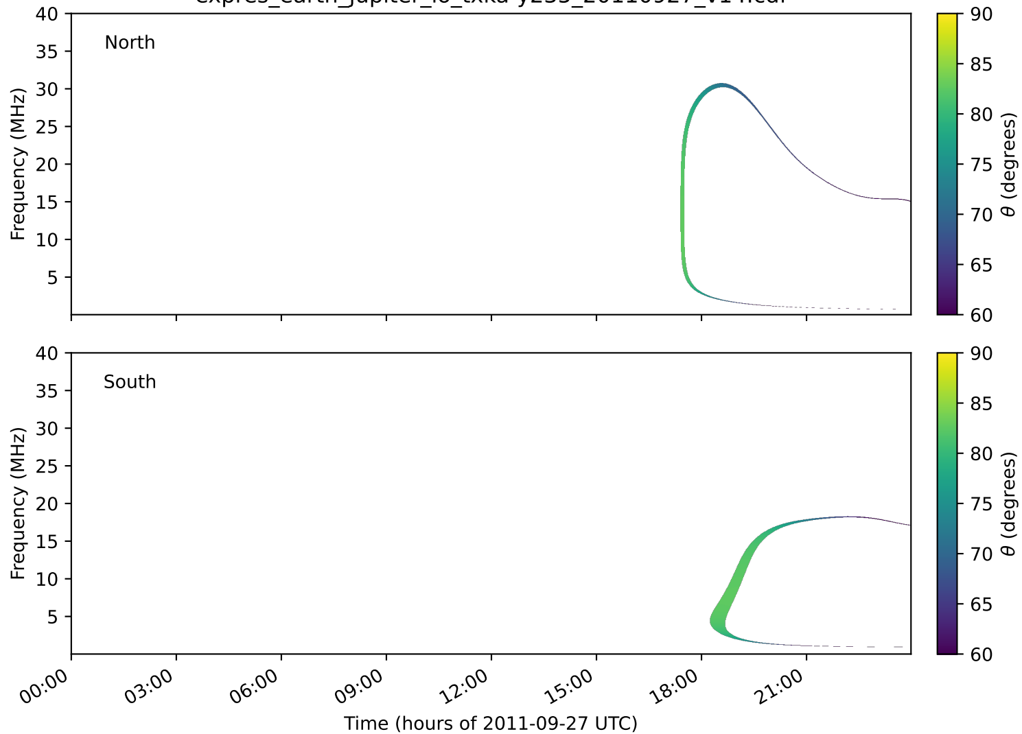
expres_earth_jupiter_io_txka-y235_20110927_v14.cdf
