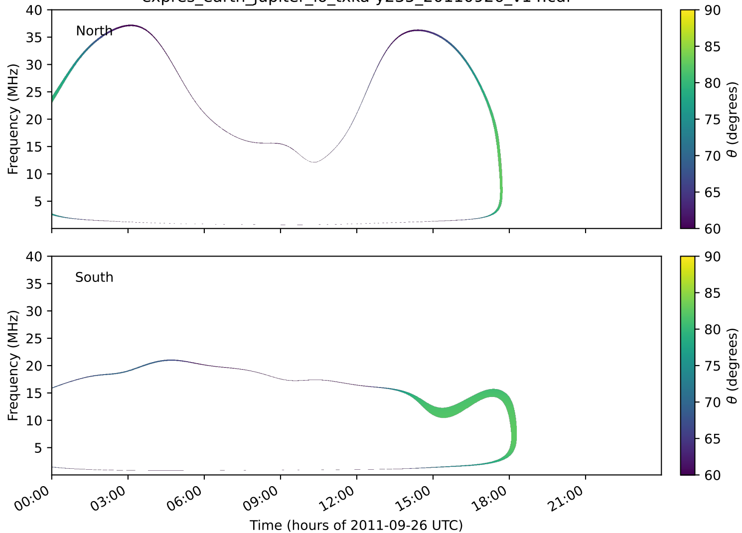
expres_earth_jupiter_io_txka-y235_20110926_v14.cdf
