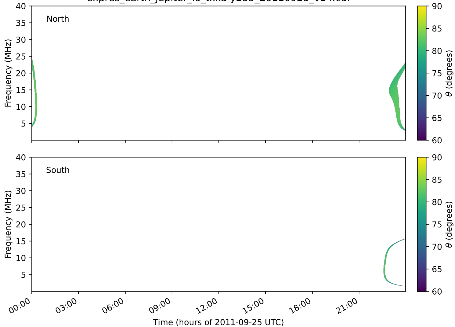
expres_earth_jupiter_io_txka-y235_20110925_v14.cdf
