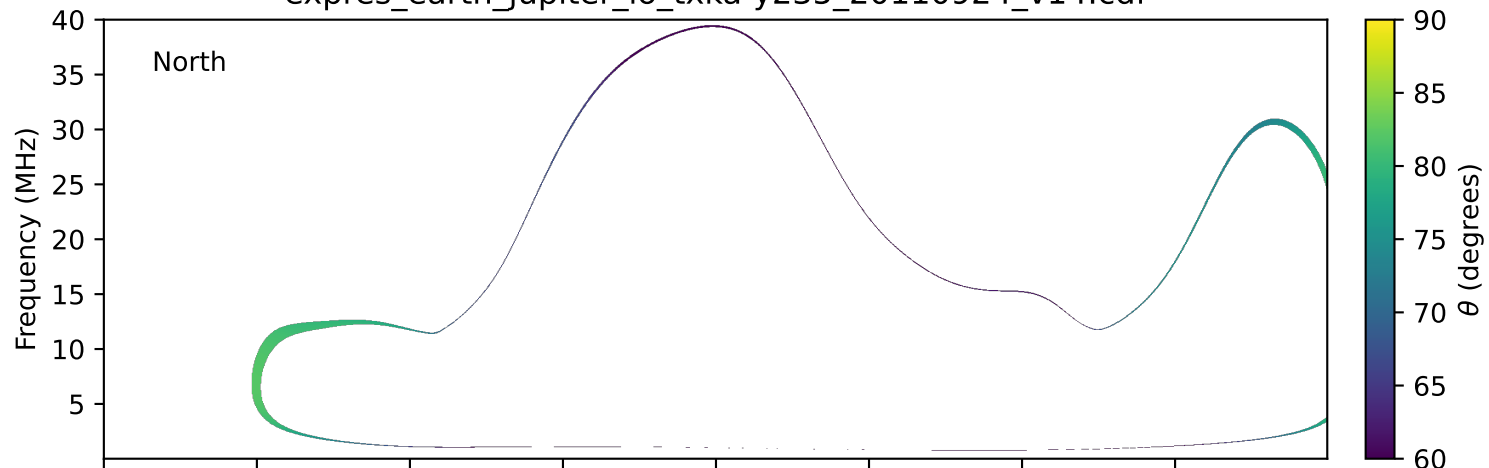
expres_earth_jupiter_io_txka-y235_20110924_v14.cdf
