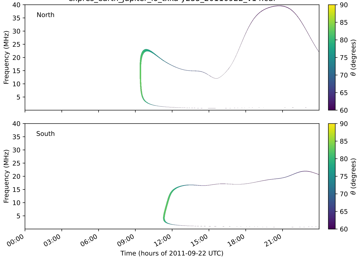
expres_earth_jupiter_io_txka-y235_20110922_v14.cdf
