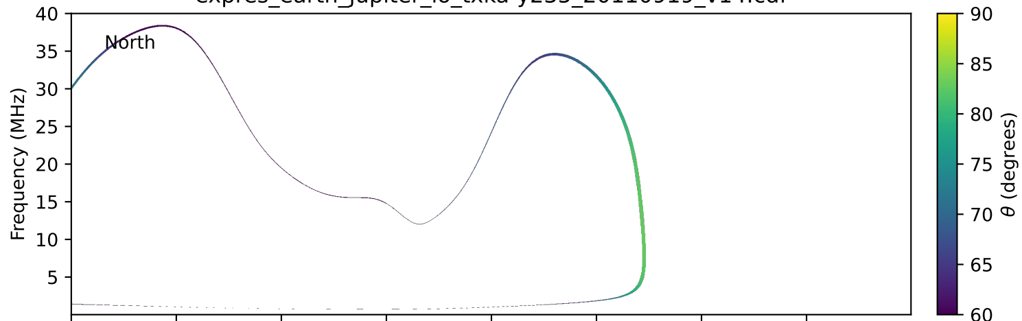
expres_earth_jupiter_io_txka-y235_20110919_v14.cdf
